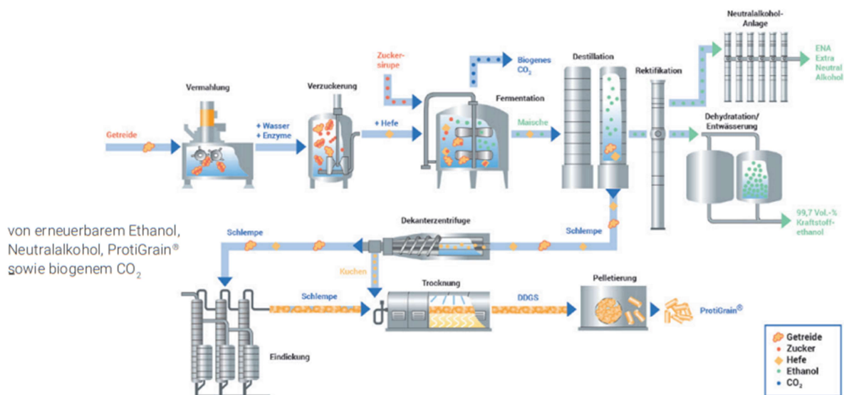
Abbildung 3: Bioraffinerie Zeitz [CropEnergies 2022]
